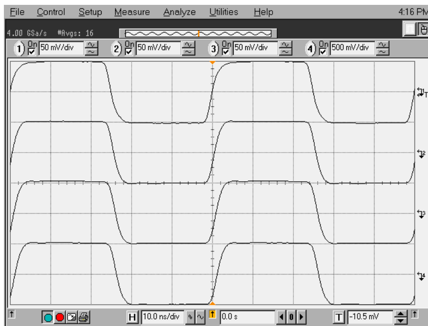
Figure 18. Broadband distribution amplifier small signal response for 20MHz square wave from Channels 1, 3, 5 & 7.
